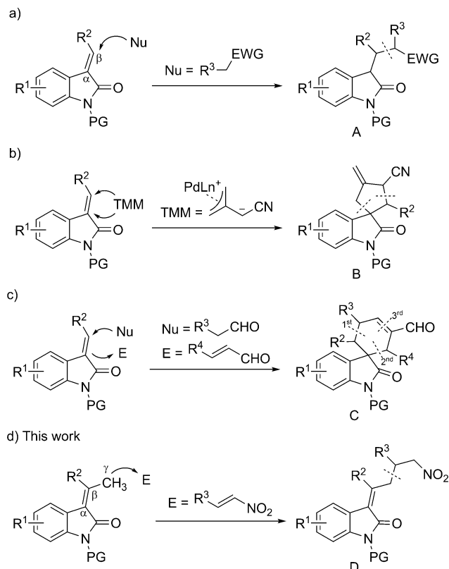
Scheme 1. Reactivity of 3-alkylidene oxindoles. a) Michael-type C_\beta functionalization. [2d,e] b) A [3+2] trimethylenemethane (TMM) cycloaddition. [2a,b] c) Michael/Michael/aldol annulation cascade. [2d,e] d) Vinylogous Michael-type C_\gamma functionalization (this work). PG = protecting group; EWG = electron-withdrawing group.
